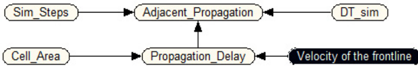
Fig. 12. Cell subnetwork implementing fire propagation control.
