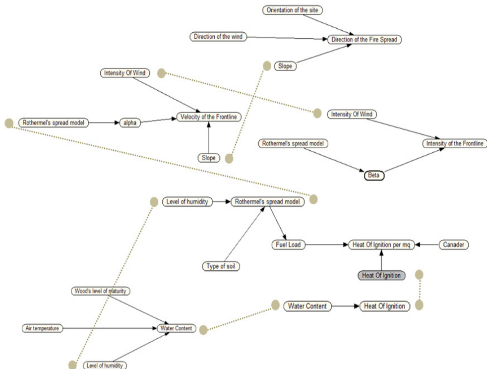
Fig. 4. Logic framework of the spatial cell of the Spatio-temporal Bayesian model
