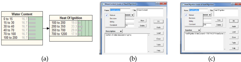
Fig. 10. Quantitative relationships among the variables
