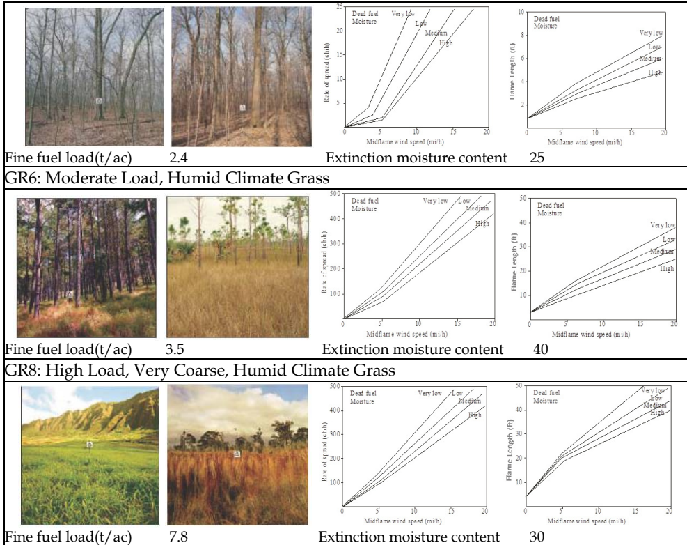
Fig. 5. Rothermel's models
