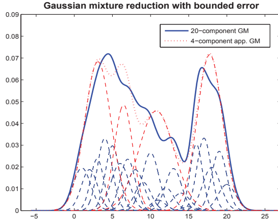
Fig. 5. Using a 4-component GM to approximate a 20-component GM with \sqrt{d} < 3\% .
