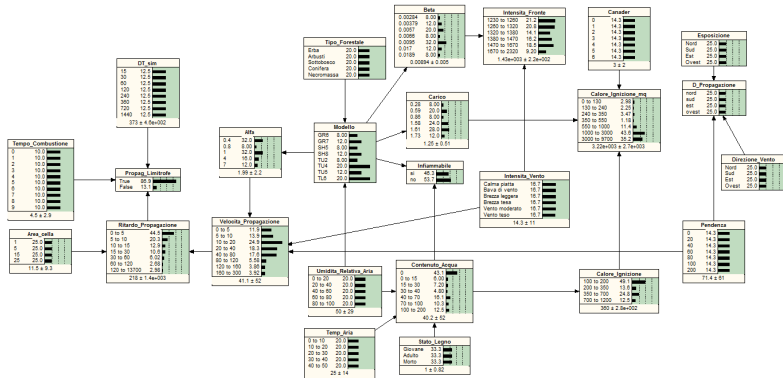
Fig. 13. Implementation of the single cell model with the Netica software
