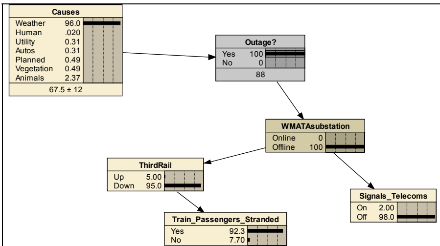
Fig. 4. A DBN with power outage
