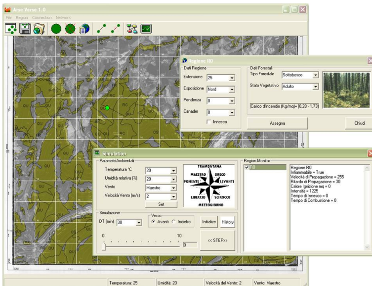
Fig. 15. The simple interface of the software prototype
