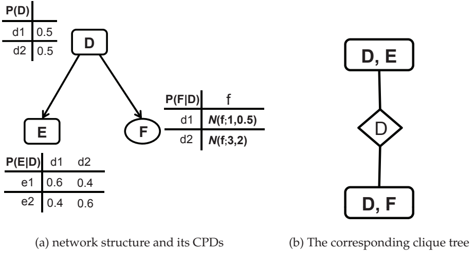
Fig. 13. A simple hybrid Bayesian network model consisting of 2 binary discrete nodes ( D, E ) and one Gaussian variable ( F ).
